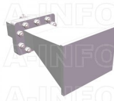
LB-229-10-C-3.5FSPO Standard Gain Horn Antenna 3.3-4.9GHz 10dB Gain 3.5mm Female
